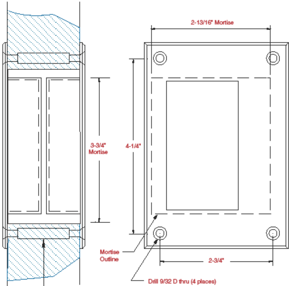
#8 Machine screw with threaded sleeve
